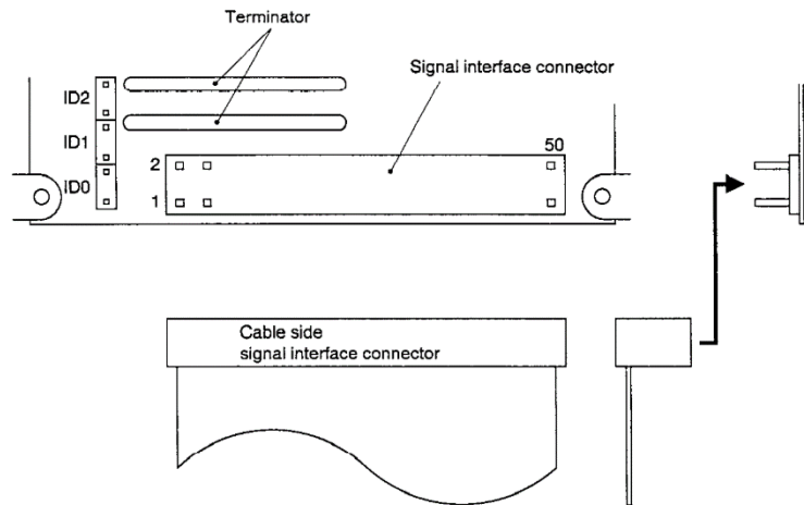
FIGURE 2, LOCATION OF FC1 TERMINATORS
