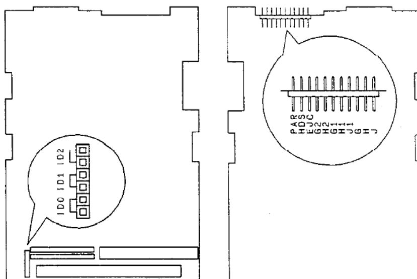
(Fig.20) Straps arrangement
