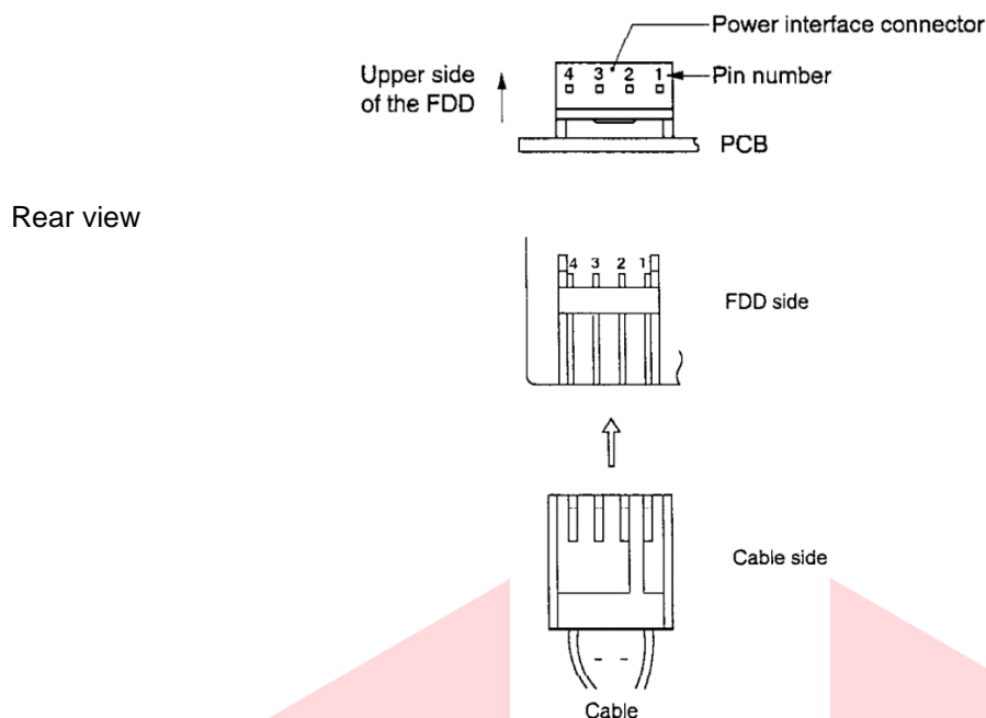
(Fig.7) Power interface connector external view
